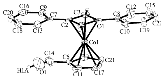
Figure 8. Thermal ellipsoid view of complex 11 with 30% probability ellipsoids (all H atoms, except those of the cyclobutadiene moiety, omitted for clarity).
