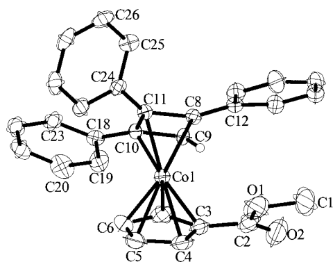
Figure 7. Thermal ellipsoid view of complex 7 with 30% probability ellipsoids (all H atoms, except those of the cyclobutadiene moiety, omitted for clarity).
