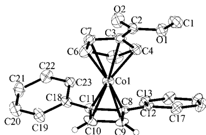
Figure 6. Thermal ellipsoid view of complex 6 with 30% probability ellipsoids (all H atoms, except those of the cyclobutadiene moiety, omitted for clarity).
