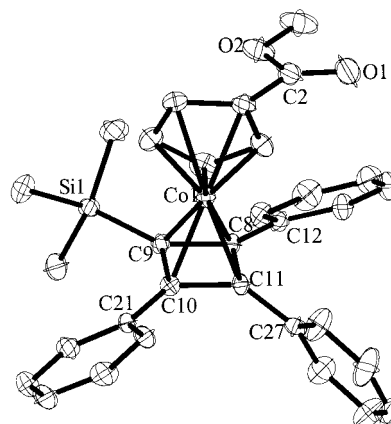
Figure 3. Thermal ellipsoid view of complex 3 with 30% probability ellipsoids (H atoms omitted for clarity).
