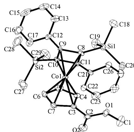
Figure 1. Thermal ellipsoid view of complex 1 with 30% probability ellipsoids (H atoms omitted for clarity).
