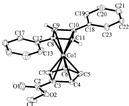
Figure 5. Thermal ellipsoid view of complex 5 with 30% probability ellipsoids (all H atoms, except those of the cyclobutadiene moiety, omitted for clarity).
