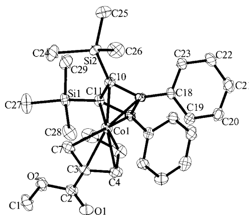
Figure 2. Thermal ellipsoid view of complex 2 with 30% probability ellipsoids (H atoms omitted for clarity).
