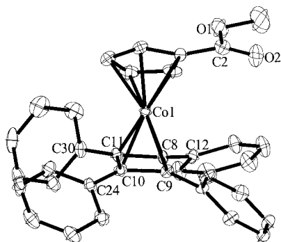
Figure 4. Thermal ellipsoid view of complex 4 with 30% probability ellipsoids (H atoms omitted for clarity).
